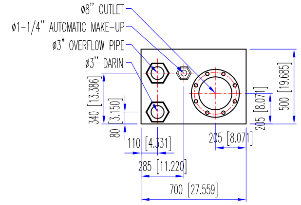
DETAIL A 1:25
