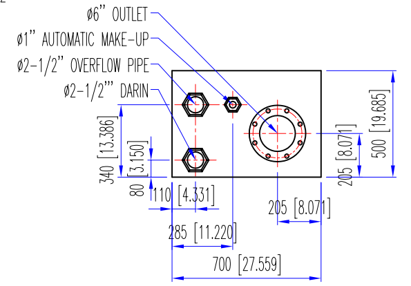
DETAIL A 1:25
